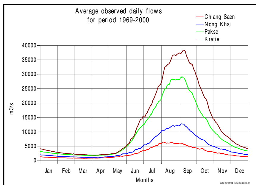
Figure 3-2. Mean daily flows at Mekong mainstream stations
