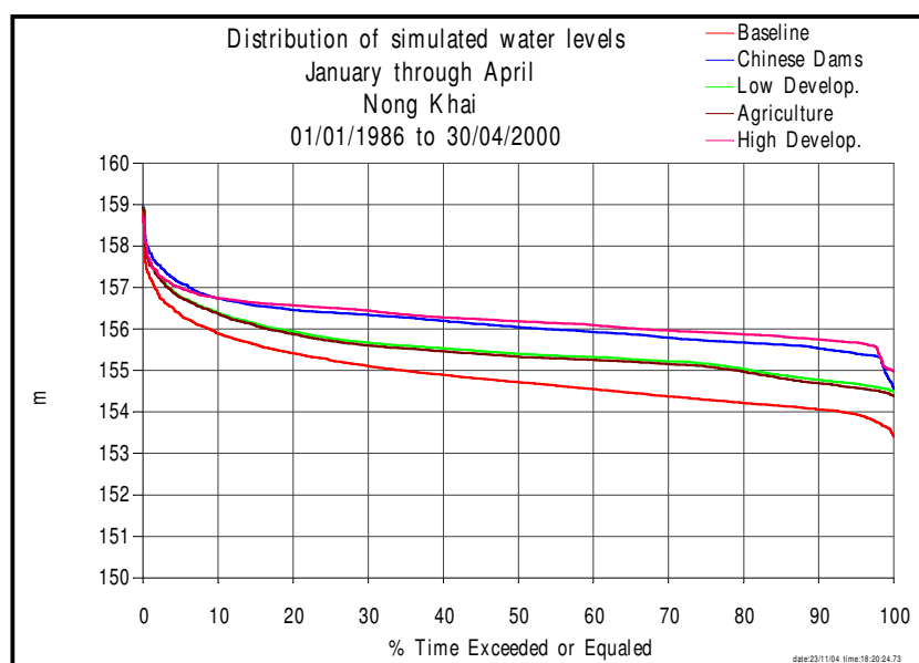
Figure 6-29. Simulated height exceeded at Nong Khai (January-April)
