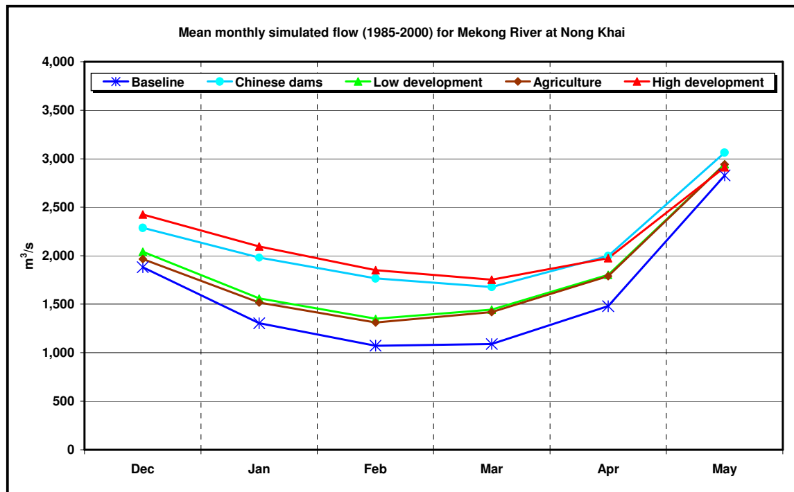
Figure 6-3. Mean monthly simulated flows at Nong Khai (1986-2000)
