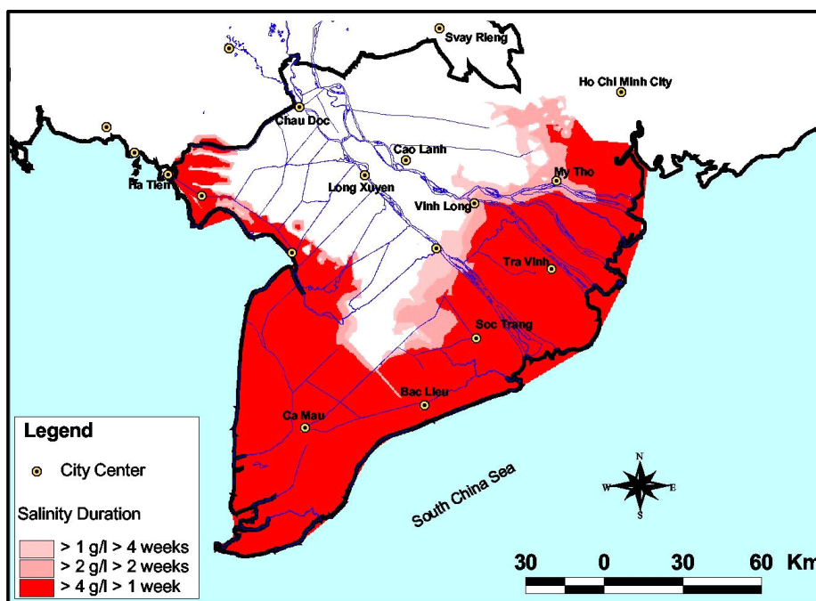
Figure 6-21. Maximum salinity intrusion for Baseline scenario - lowest flow year 1998
