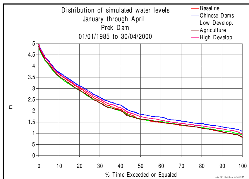
Figure 6-32. Simulated height exceeded at Prek Dam (January-April)
