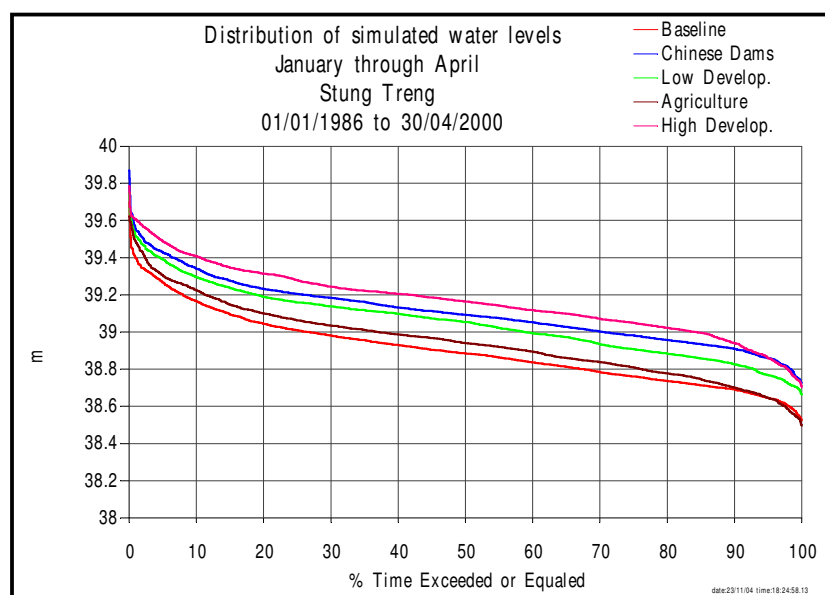
Figure 6-30. Simulated height exceeded at Stung Treng (January-April)
