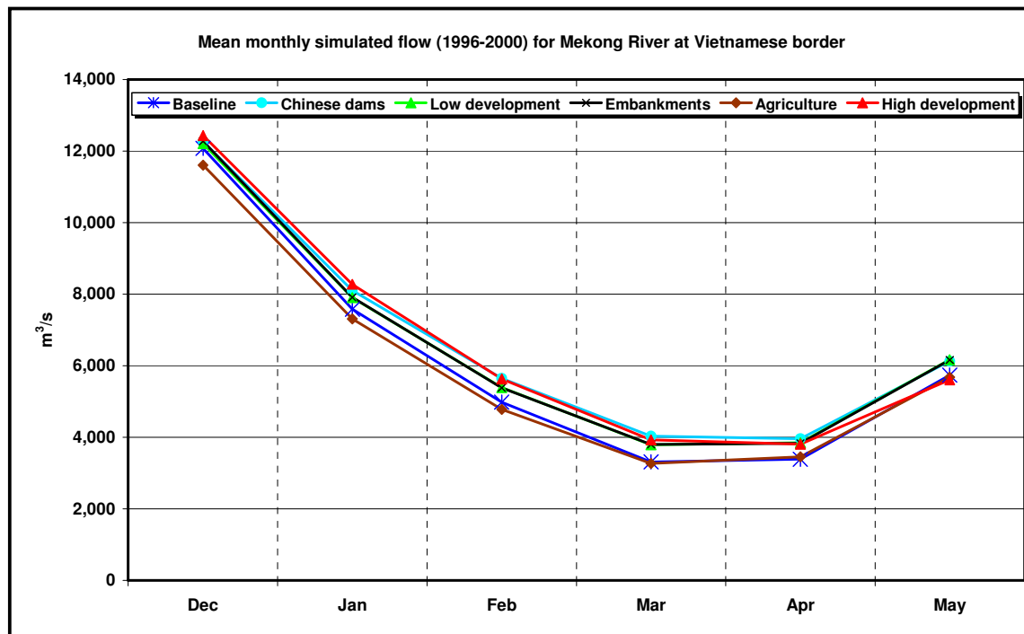
Figure 6-6. Mean monthly simulated cross boundary flows into the Mekong Delta (1996-2000)
