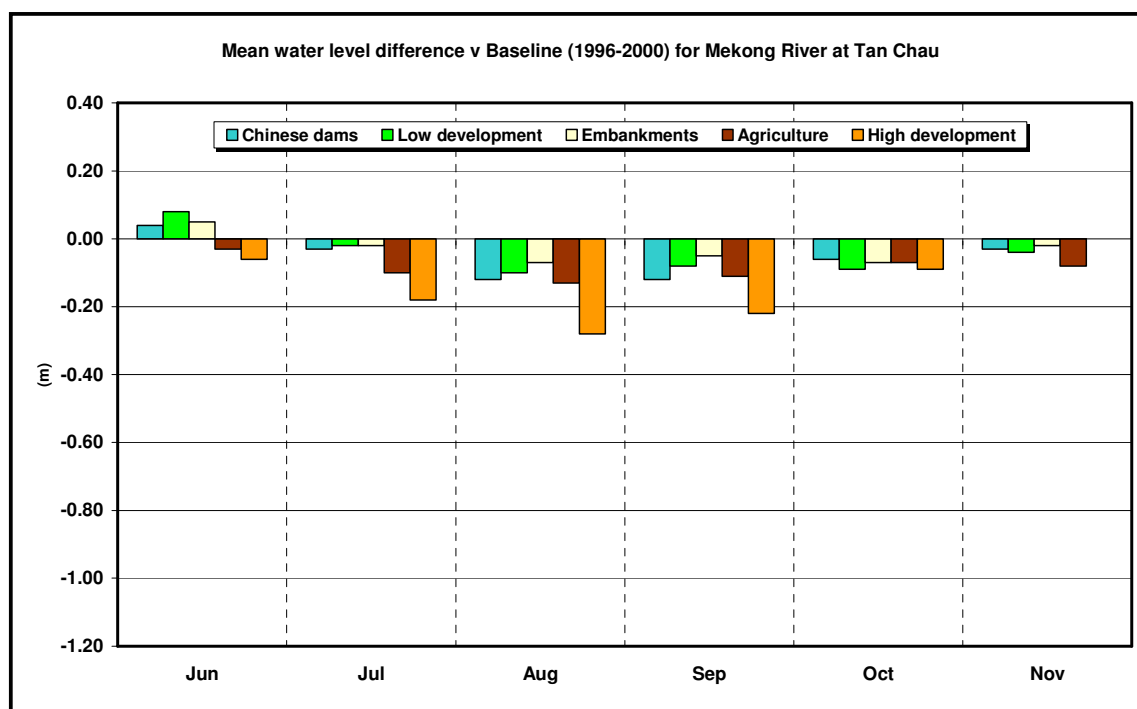
Figure 6-10. Change in mean monthly simulated water level at Tan Chau (1996-2000)
