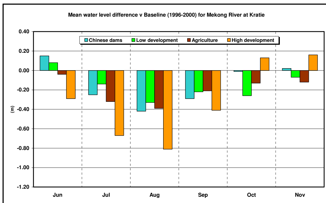
Figure 6-9. Change in mean monthly simulated water level at Kratie (1996-2000)
