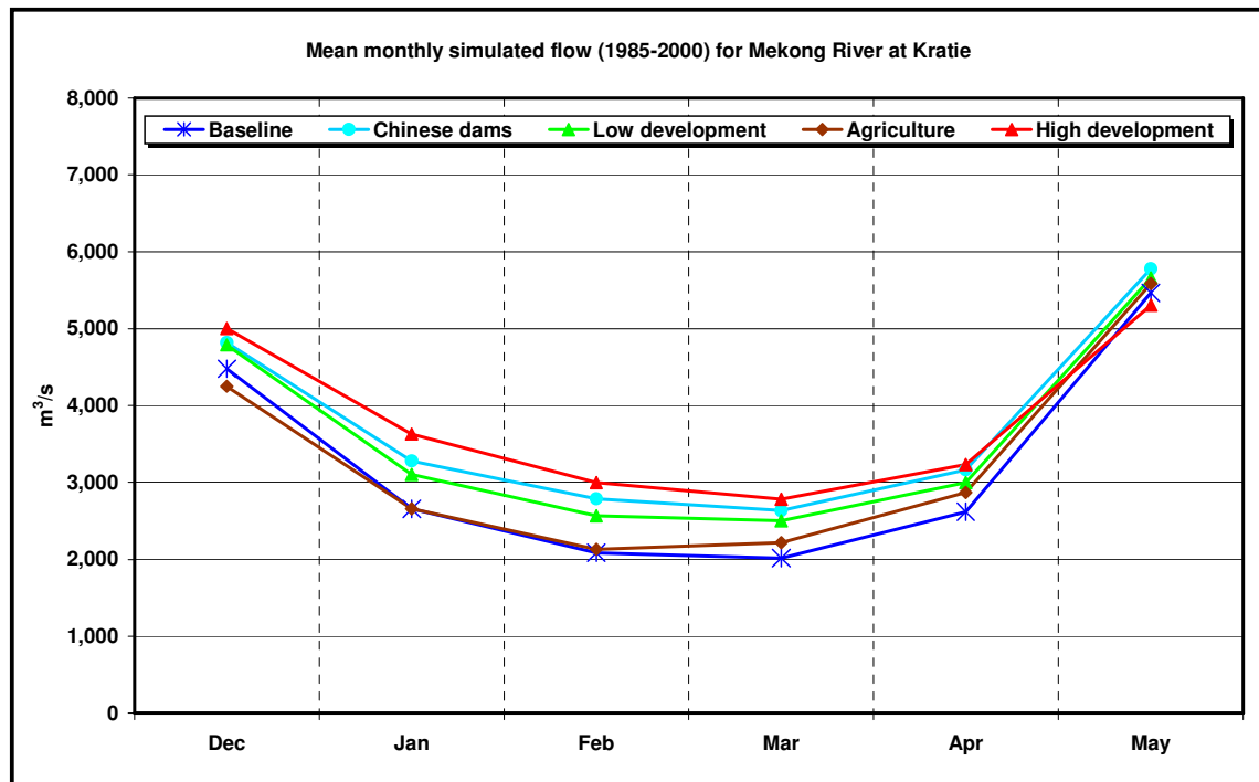
Figure 6-5. Mean monthly simulated flows at Kratie (1986-2000)
