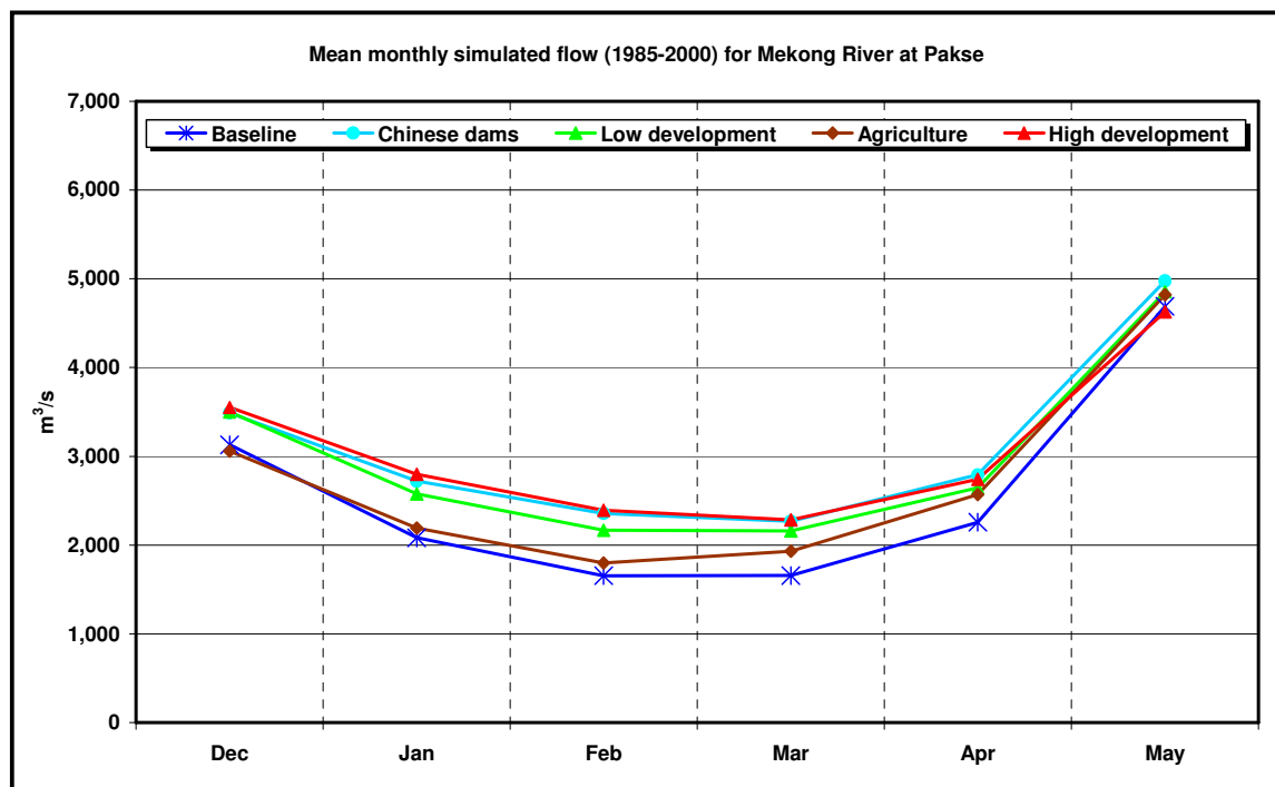
Figure 6-4. Mean monthly simulated flows at Pakse (1986-2000)
