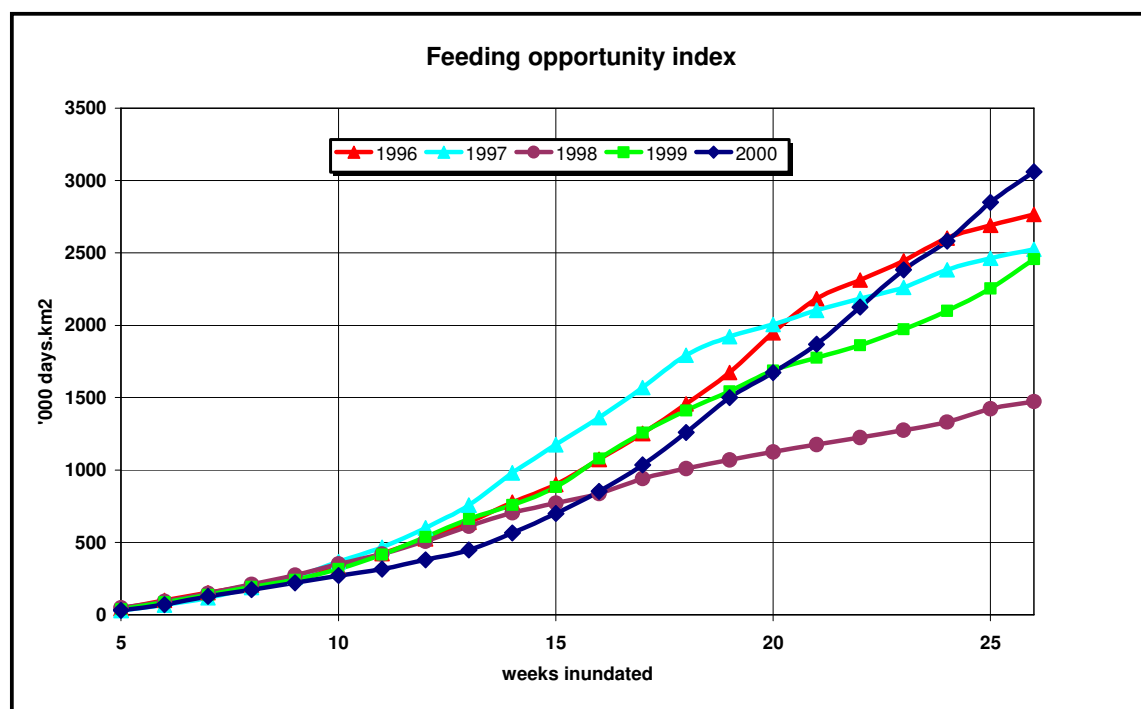
Figure 6-27. Feeding Opportunity Index for different periods inundated-Baseline scenario
