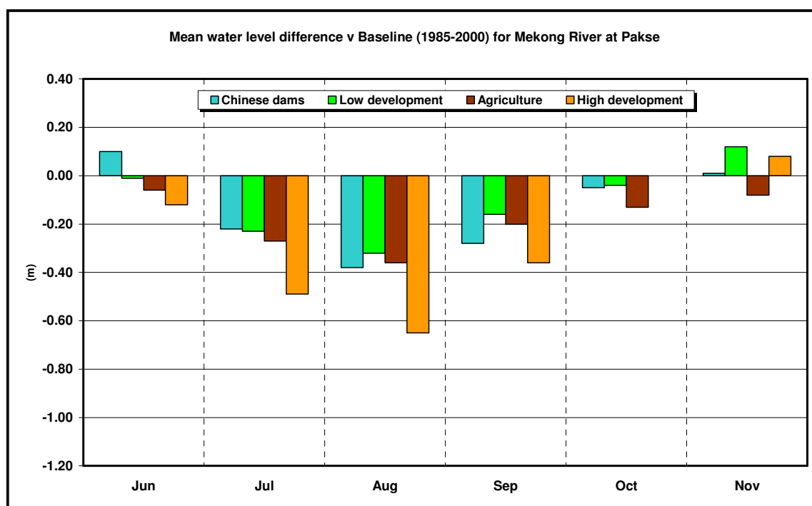
Figure 6-8. Change in mean monthly simulated water level at Pakse (1986-2000)
