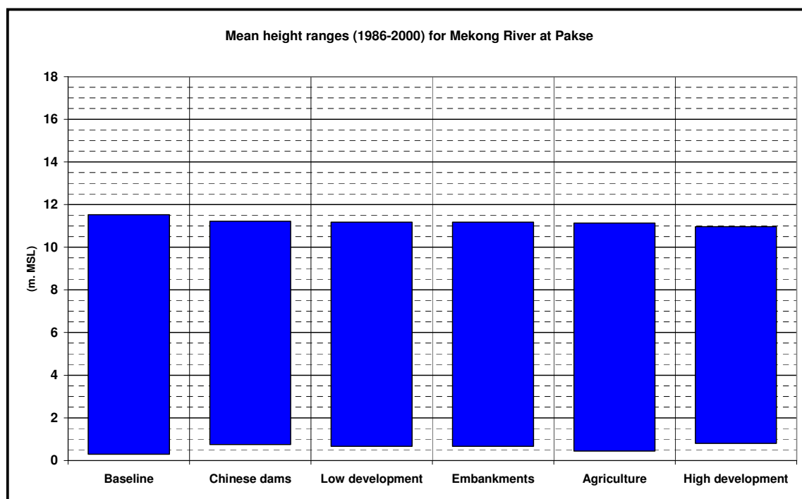
Figure 6-12. Mean maximum and minimum simulated water levels at Pakse (1986-2000)
