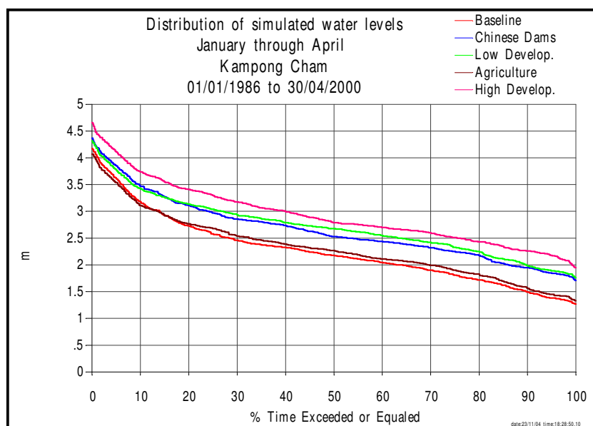
Figure 6-31. Simulated height exceeded at Kampong Cham (January-April)
