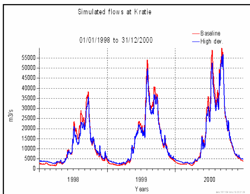
Figure 7-2. Simulated flows at Kratie: 1998-2000: Baseline v High Development scenarios
