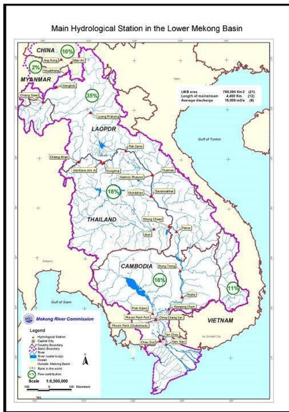
Figure 1. Mainstream hydrographic stations and country flow contributions for the LMB
