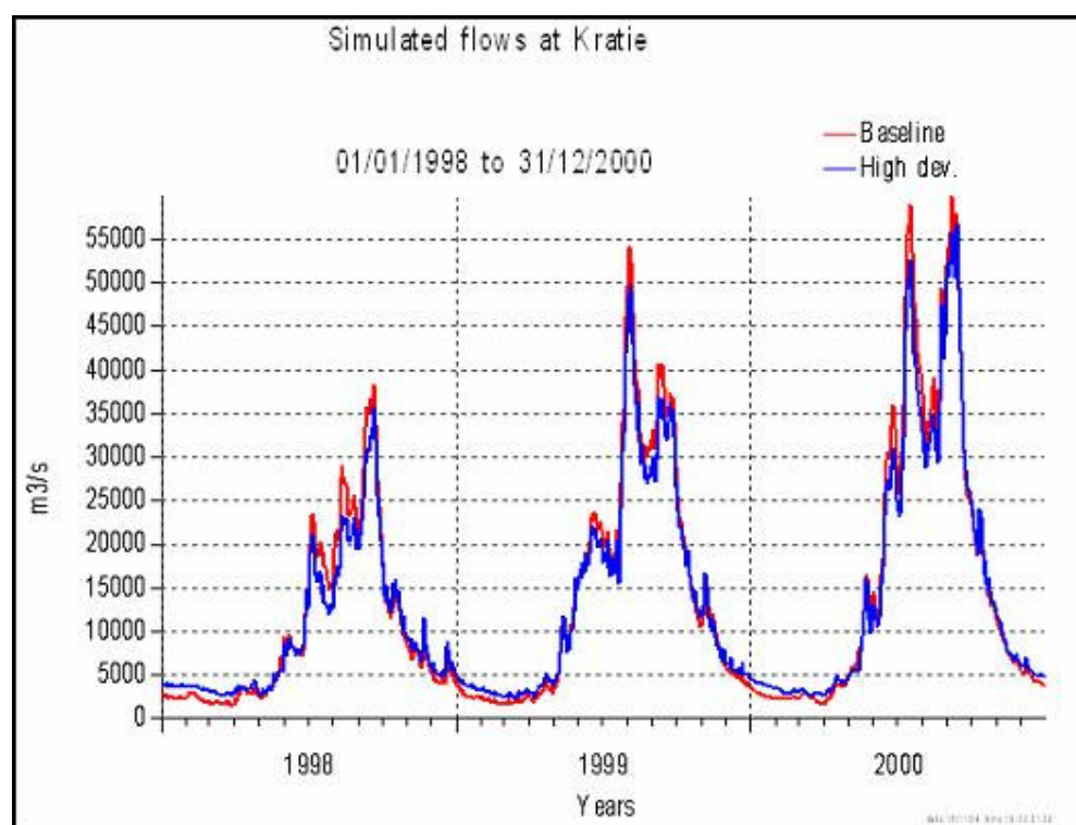
Figure 3. Simulated flows at Kratie
