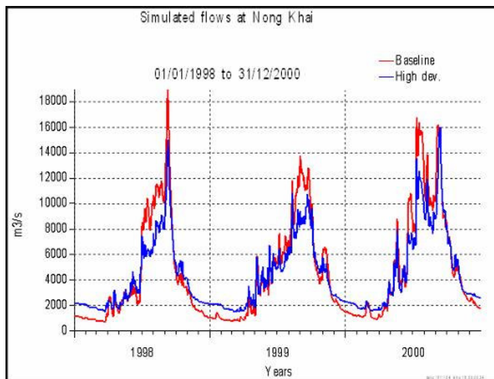
Figure 2. Simulated flows at Nong Khai
