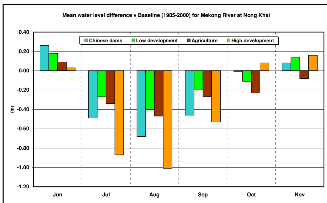
Figure 6-7. Change in mean monthly simulated water level at Nong Khai (1986-2000)
