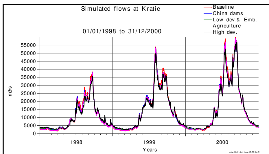
Figure 6-2. Simulated flows at Kratie 1998-2000
