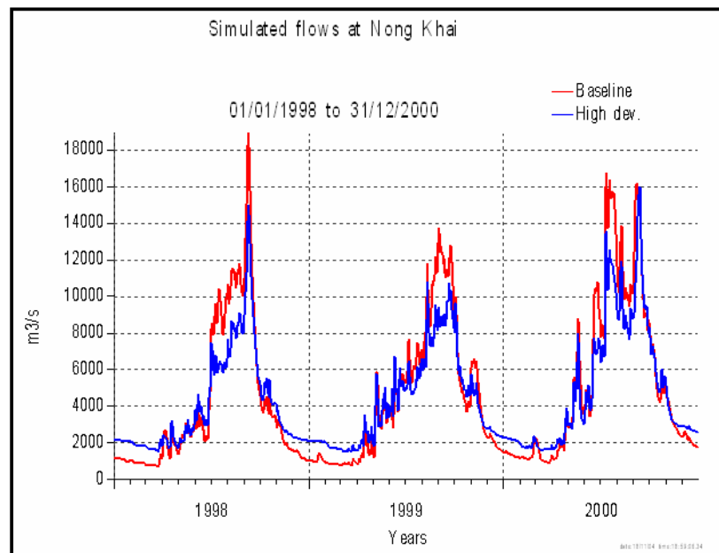
Figure 7-1. Simulated flows at Nong Khai 1998-2000: Baseline v High Development scenarios
