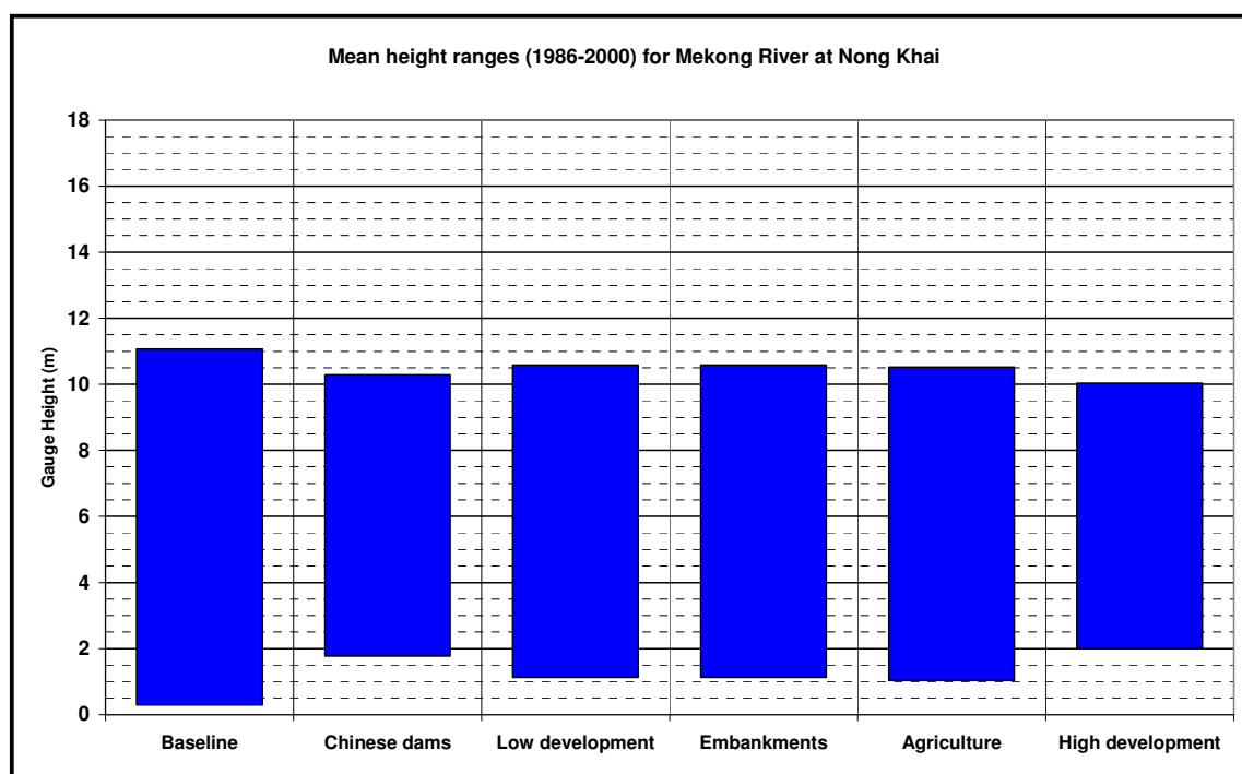
Figure 6-11. Mean maximum and minimum simulated water levels at Nong Khai (1986-2000)
