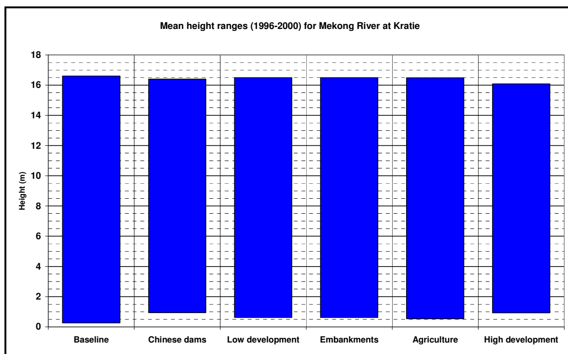
Figure 6-13. Mean maximum and minimum simulated water levels at Kratie (1996-2000)
